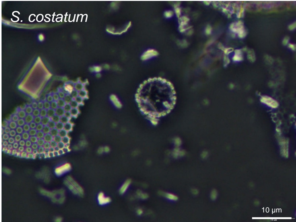
Peru upwelling
