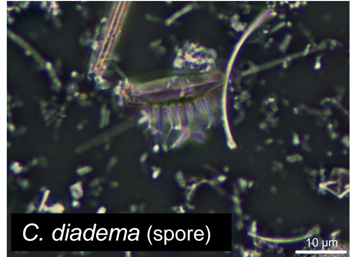
Peru upwelling
