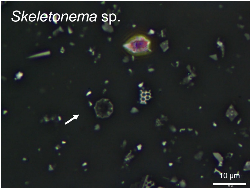
Peru upwelling
